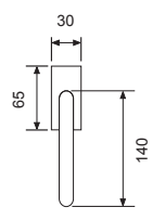
33080DK - RAL 9005 Tilt and turn handle DK
