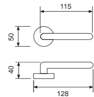
23066R04 - ZCS Handle on rose Maner cu rozeta
