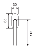
33066DK - ZCS Tilt and turn handle DK
