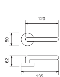
21058R03 - OBG Handle on rose Maner cu rozeta
