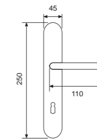
21034P - OBG Handle on plate Maner cu placa
