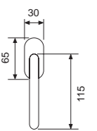
33050DK - ZCS Tilt and turn handle DK
