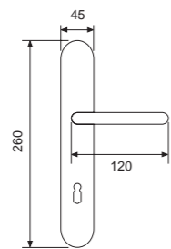
21058P - OBG Handle on plate Maner cu placa
