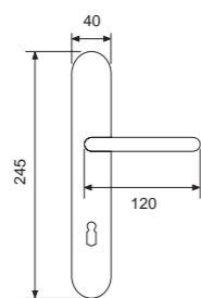
21018P - OLV Handle on plate Maner cu placa
