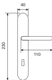
21023P - OLV Handle on plate Maner cu placa
