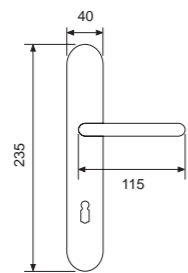
21024P - OLV Handle on plate Maner cu placa
