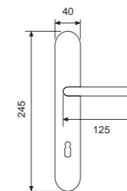
21064P - OLV Handle on plate Maner cu placa
