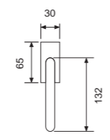
23088DK - ZCS Tilt and turn handle DK
