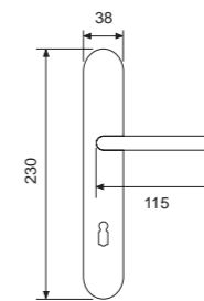
21072P - OCL/OCS Handle on plate Maner cu placa
