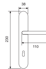
21069P - OCS Handle on plate Maner cu placa
