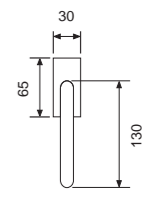
33070DK - ZCS Tilt and turn handle DK
