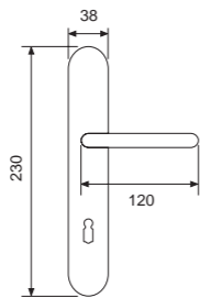
21089P - OCS Handle on plate Maner cu placa
