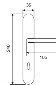
21292P - OLV Handle on plate Maner cu placa
