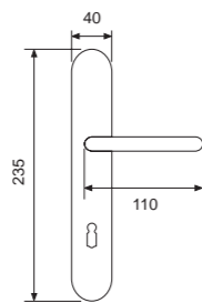
21026P - OLV Handle on plate Maner cu placa
