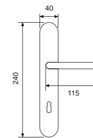
21052P - ONS Handle on plate Maner cu placa
