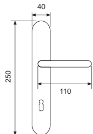
21046P - OBV Handle on plate Maner cu placa
