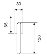
23084DK - ZCS Tilt and turn handle DK
