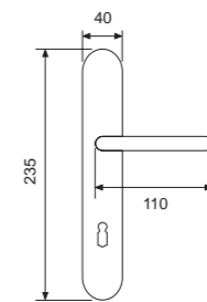
21057P - OLV Handle on plate Maner cu placa
