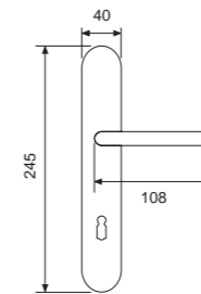
21078P - OLV Handle on plate Maner cu placa
