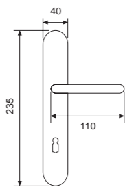
21077P - OLV Handle on plate Maner cu placa
