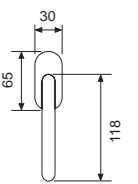
33062DK - ZCS Tilt and turn handle DK
