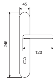
21016P - OCS Handle on plate Maner cu placa
