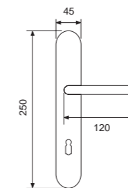
21070P - OBG Handle on plate Maner cu placa
