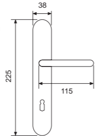
23066PF - ZCS Handle on plate Maner cu placa
